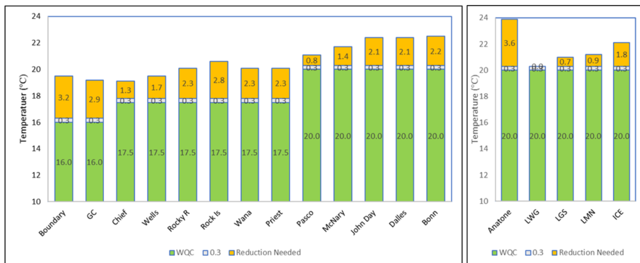
Figure 6-2 Comparing measured maximum monthly temperatures to the target temperatures – August
