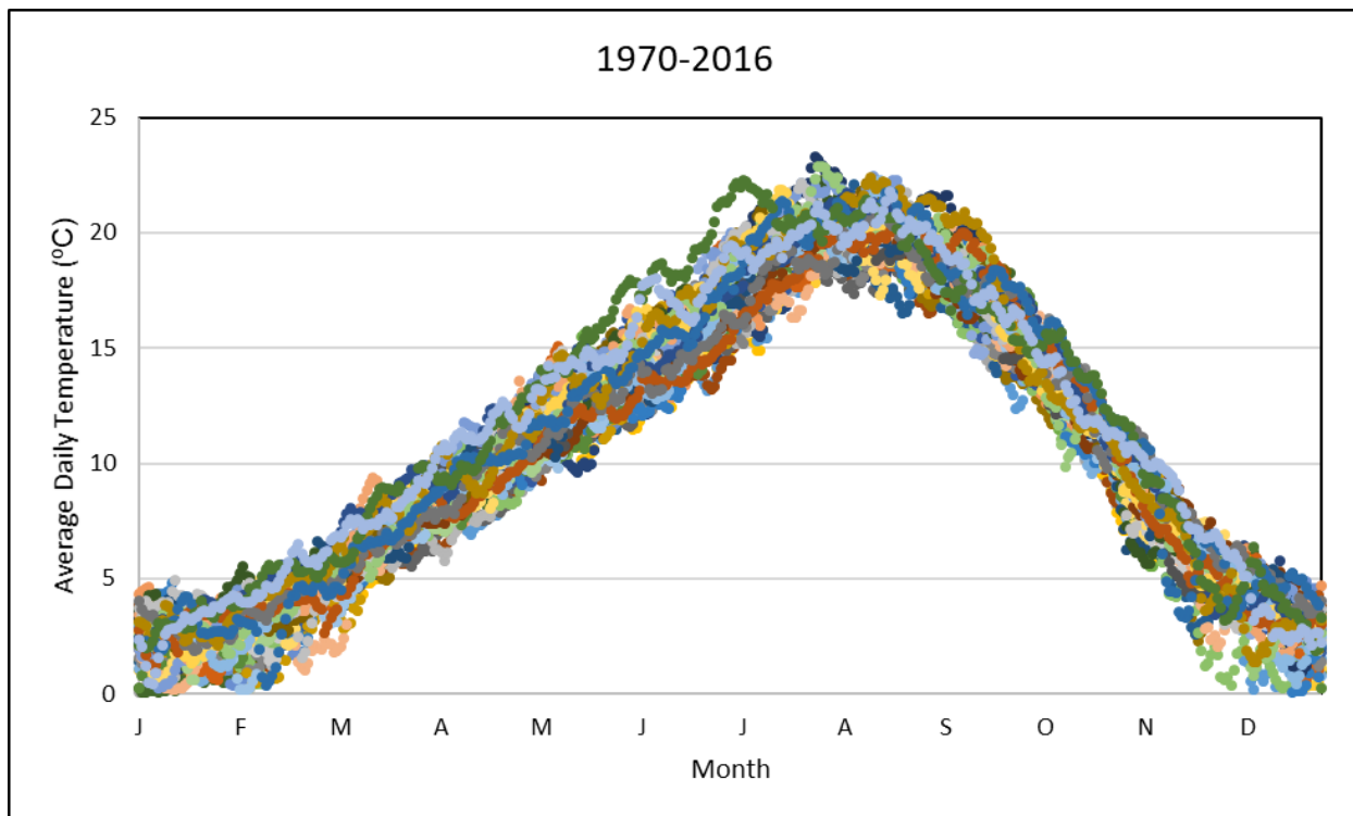
Figure 6-5 RBM10 simulation of free-flowing river temperatures at Bonneville Dam on the Columbia River (all years: 1970 – 2016)
