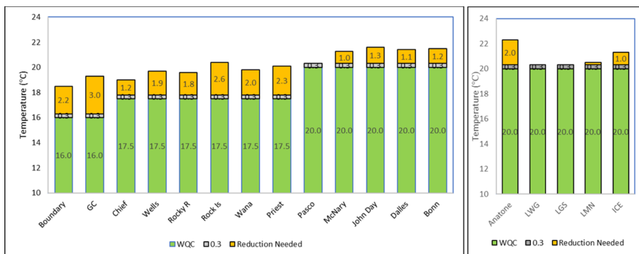
Figure 6-3 Comparing measured maximum monthly temperatures to the target temperatures – September
