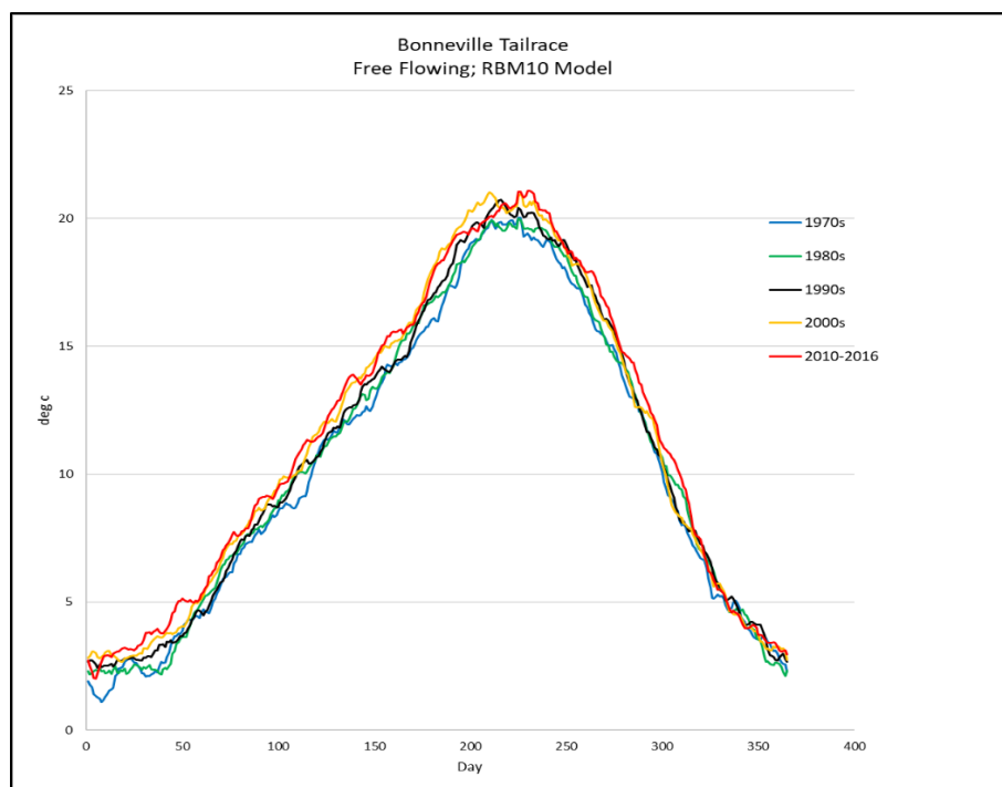
Figure 6-6 Decadal average temperatures from 47-year RBM10 simulation of free-flowing river at Bonneville Dam
