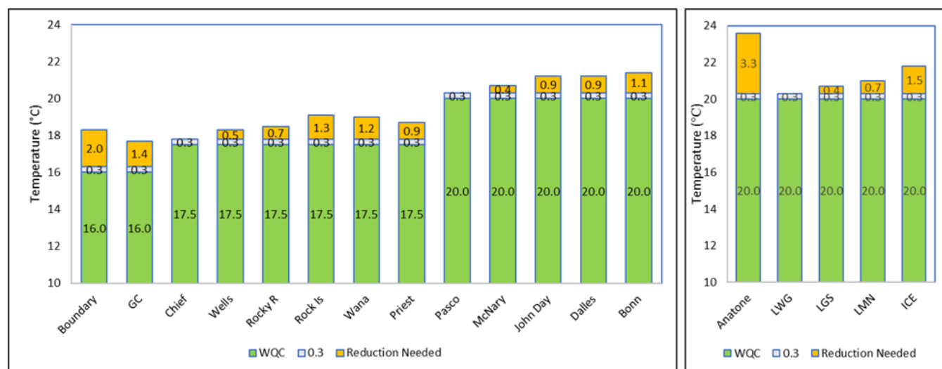
Figure 6-1 Comparing measured maximum monthly temperatures to the target temperatures – July
