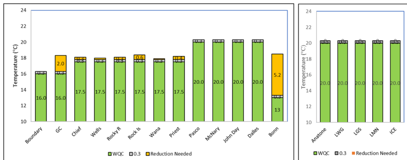
Figure 6-4 Comparing measured maximum monthly temperatures to the target temperatures – October
